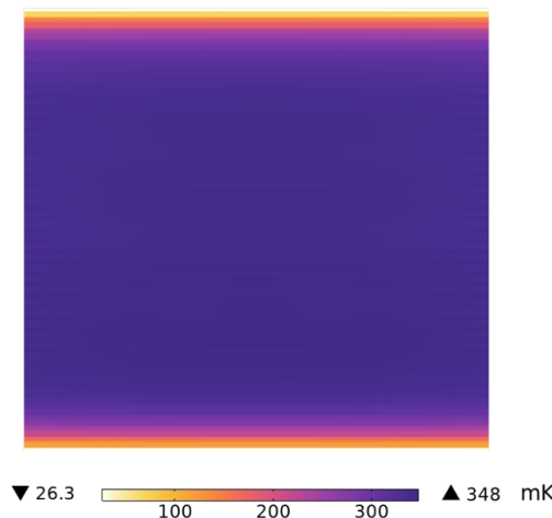
Fig. 10. Temperature distribution on the central-upper stack with 5 \times 10^{-3} Km 2 /W contact resistance between all the layer interfaces. The temperature is higher and more homogenous in the central part, while steeper gradients arise at the upper and bottom periphery of the stack. Despite these differences, no dangerous peak is reached.
