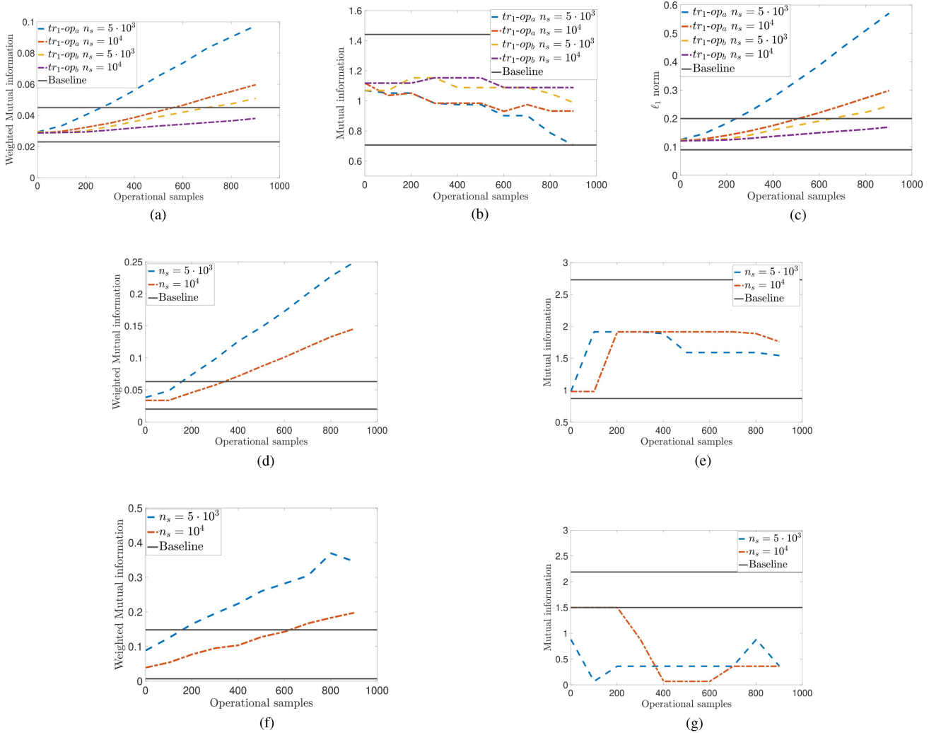
Fig. 2. Incremental groupwise results. (a) RUL tr_1-op_a and tr_1-op_b with W\mu I . (b) RUL tr_1-op_a and tr_1-op_b with \mu I . (c) RUL tr_1-op_a and tr_1-op_b with l_1 norm. (d) Platooning with W\mu I . (e) Platooning with \mu I . (f) DNS with W\mu I . (g) DNS \mu I .
