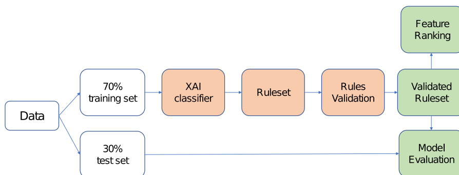
Fig 1. Workflow of the analyses carried out in the proposed XAI-based approach.
