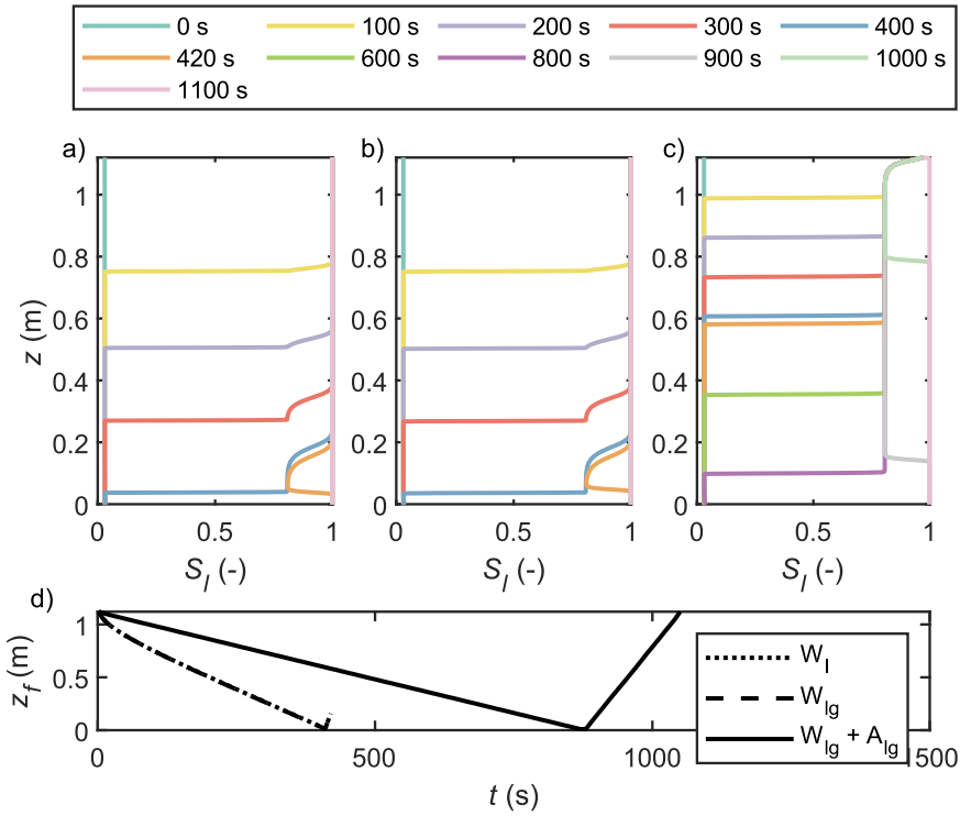
Fig. 3. a-c) Profiles of liquid-phase saturation degree S_l for different time instants, for a) “ W_l ” model, b) “ W_{lg} ” model and c) “ W_{lg}+A_{lg} ” model; d) Temporal evolution of the location of the wetting/saturation front, labeled as z_f .
