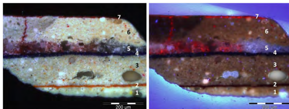
Figure 3. Paint stratigraphy, cross section from Inv. 450. Polarized light (left) and UV (right) images of a cross section from Inv. 450; the sequence of paint layers includes (1) lithopone with sparse calcium carbonate inclusions and earth pigments, (2) minium, (3) lithopone with sparse earth pigments, (4) ultramarine blue, (5) red lake with calcium carbonate substrate, (6) lithopone with sparse earth pigments, and (7) red lake with aluminum and iron silicate substrate.
