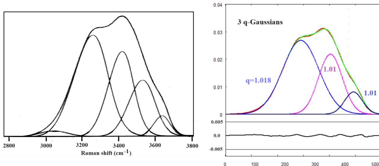
Fig. 3: Left - Sketch adapted from the Figure 9 by Carey, 1996, giving the “Gaussian deconvoluted vibrational Raman spectrum of liquid water at 24°C and 128 Bar pressure”. In the caption, Carey is mentioning five Gaussian peaks, postulated as a Fermi resonance at 3050\text{ cm}^{-1} and four \nu_1 symmetrical stretching vibrations at \sim 3240 , \sim 3390 , \sim 3490 , and \sim 3627\text{ cm}^{-1} . For what is regarding the Fermi resonance, see please again Maeda and Kitano, mentioning Hare and Sorensen, 1992. Right - Decomposition with three q-Gaussians.
