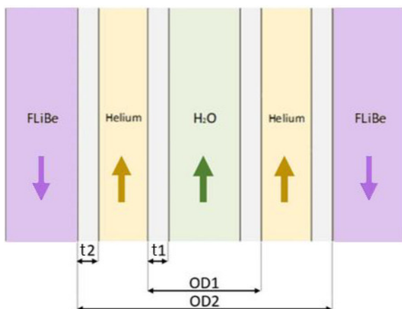
Fig. 1. Double Wall Tube radial section.
