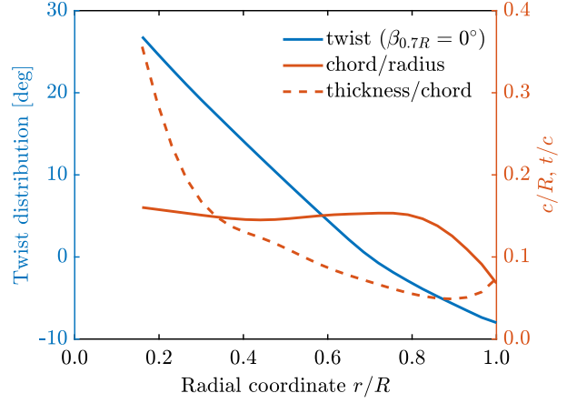
(b) Propeller blade geometry
