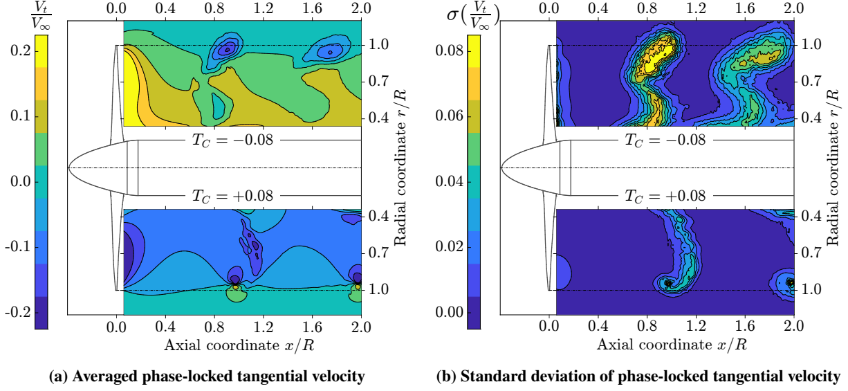
Fig. 19 Comparison of tangential velocity contours in negative ( \beta_{0.7R} = 20^\circ ) and positive ( \beta_{0.7R} = 38.93^\circ ) thrust condition at absolute thrust level of |T_C| = 0.08 (Phase-locked)
