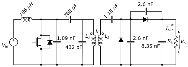
Fig. 7. Schematic of the class-E-DE converter based on inductive coupling taken from [12]
