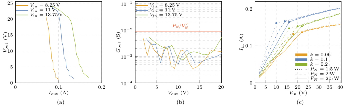
Fig. 6. Characteristics of the classical class-E 2 DC-DC converter based on capacitive coupling: (a) output curves of the converter for three different input voltages from which the current source behaviour becomes clear; (b) output conductance of the converter compared to that of the nominal load in order to justify the use of a shunt regulator; (c) characteristics observed at the primary side of the DC-DC isolated converter for three different coupling factor values k = 0.06 , k = 0.1 , k = 0.2 and three different nominal power levels P_N = 1.5 W, P_N = 2 W, P_N = 2.5 W. The bullet points indicate the MET point identified according to the algorithm proposed in [13].
