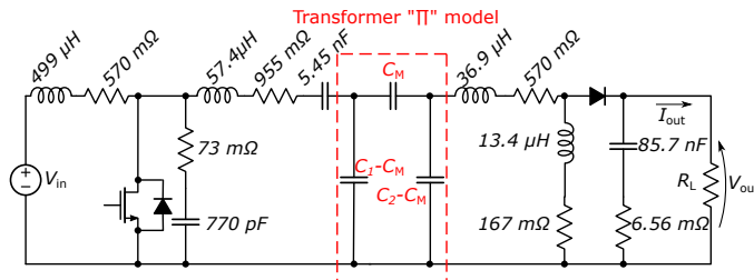
Fig. 5. Schematic of the class-E 2 DC-DC converter based on capacitive coupling taken from [3].
