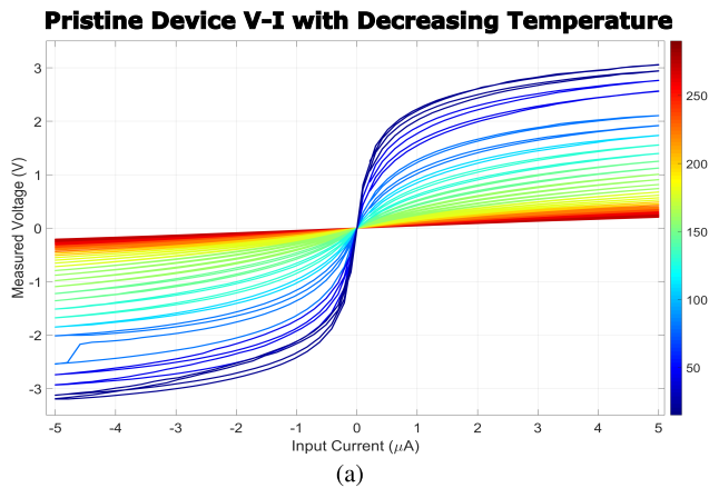
Pristine Device T vs. R Decreasing Temperature
