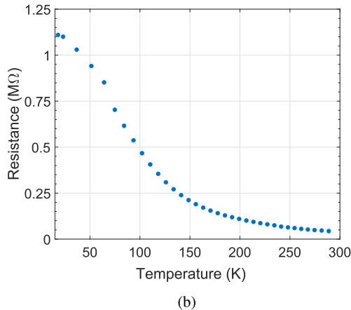
Fig. 7. Pristine device with current input in decreasing temperature (a) showing the V-I plot and (b) showing the variation of resistance.
