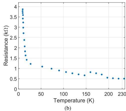
Fig. 8. Device set to LRS with current input in decreasing temperature (a) showing the V-I plot and (b) showing the variation of resistance.
