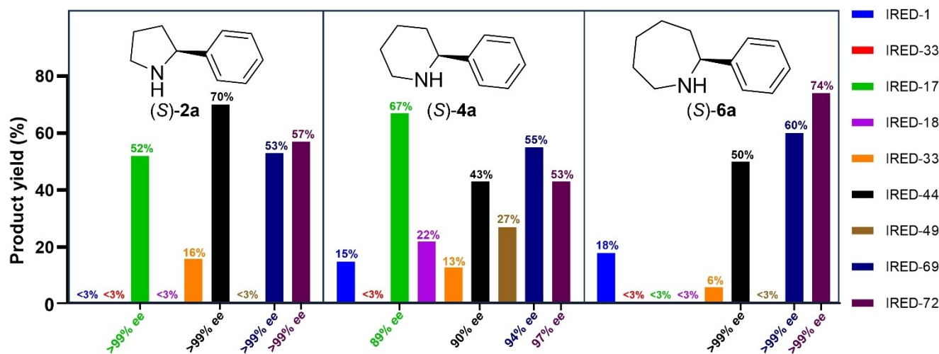
Figure 4. IRED screening for the asymmetric reduction of substrates 1a , 3a and 5a . Reaction conditions: D-glucose (100 mg), NADP + (6.4 mg), GDH-101 (6.0 mg) selected IRED (12.0 mg), imine substrate (0.14 mmol, 100 mM) added in DMF (30 \mu L), stirred (700 rpm) at 30 °C for 4 h in PB/Gly 50:50 (1.4 mL) (PB: potassium phosphate buffer 100 mM, pH 8). Yields determined by quantitative 1 H NMR analysis. %ee values (from 89% to > 99%) were determined by Chiral-HPLC analysis when the reaction showed appropriate conversion (see Supporting Information). Absolute configurations were determined by \alpha_D values measured at 25 °C.
