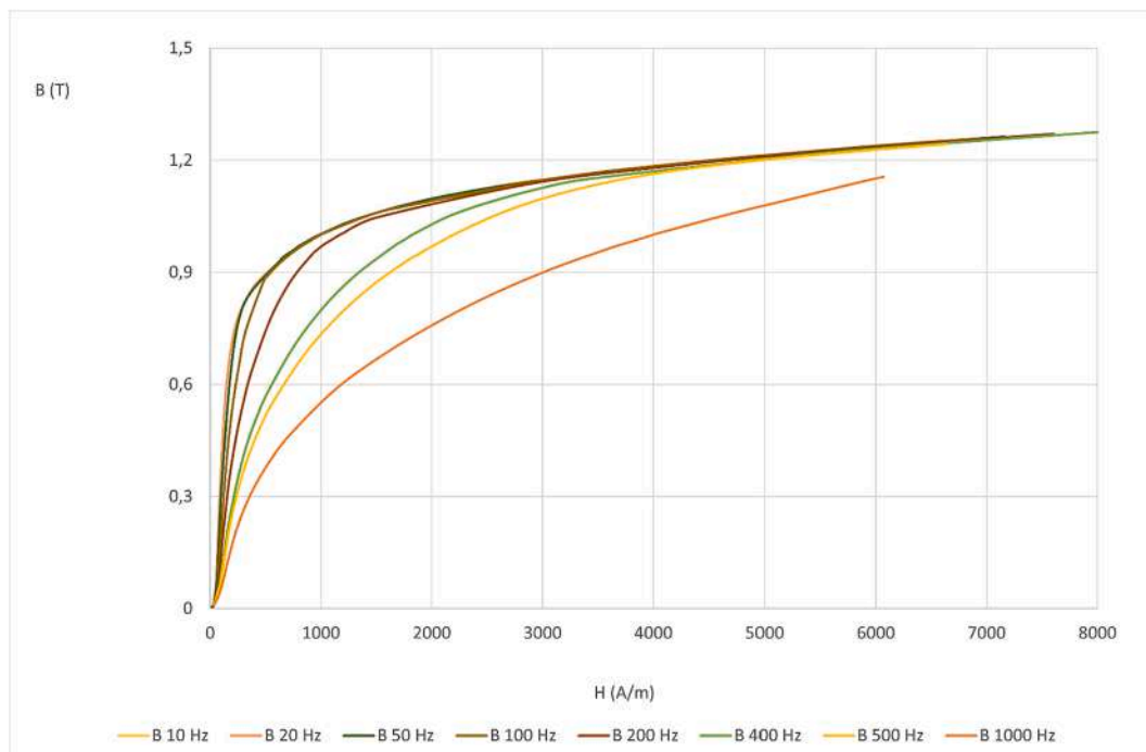
Fig. 5. Magnetization curves at different frequencies after heat treatment at 1200 °C.
