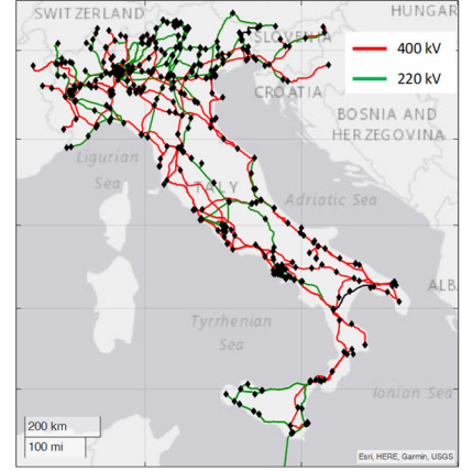
Fig. 4. Italian HV Transmission Grid with cross-border connections.
