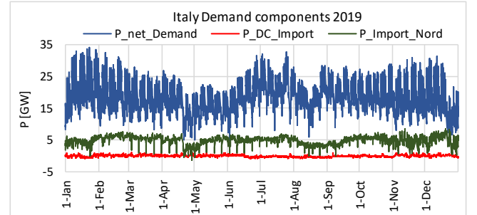
Fig. 5. Italian HV Transmission Grid demand components.
