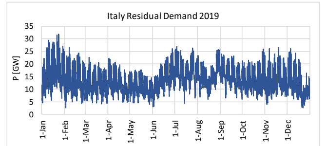
Fig. 6. Italian HV Transmission Grid residual demand.
