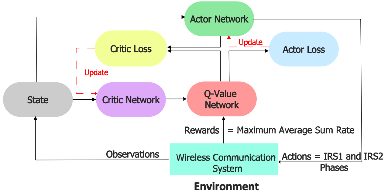
Fig. 2: DDPG model
