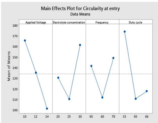
Fig. 7 Main effect plot for circularity at entry
