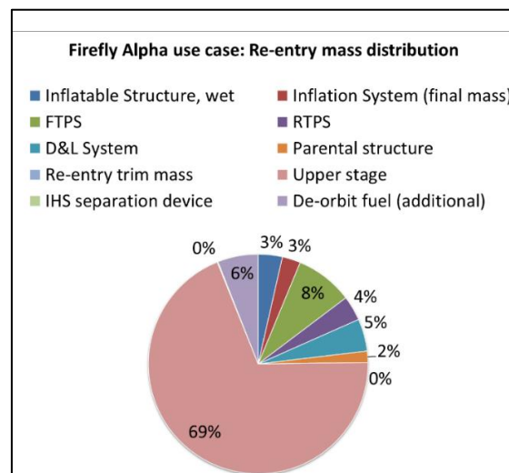
Figure 16: Mass distribution of the reference configuration during re-entry.
