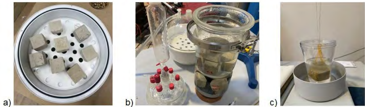
Figure 7. Some steps in the porosity calculation procedure: a) placement of samples in the desiccator b) keeping the samples immersed in water for at least 24 h c) final weighing in water
