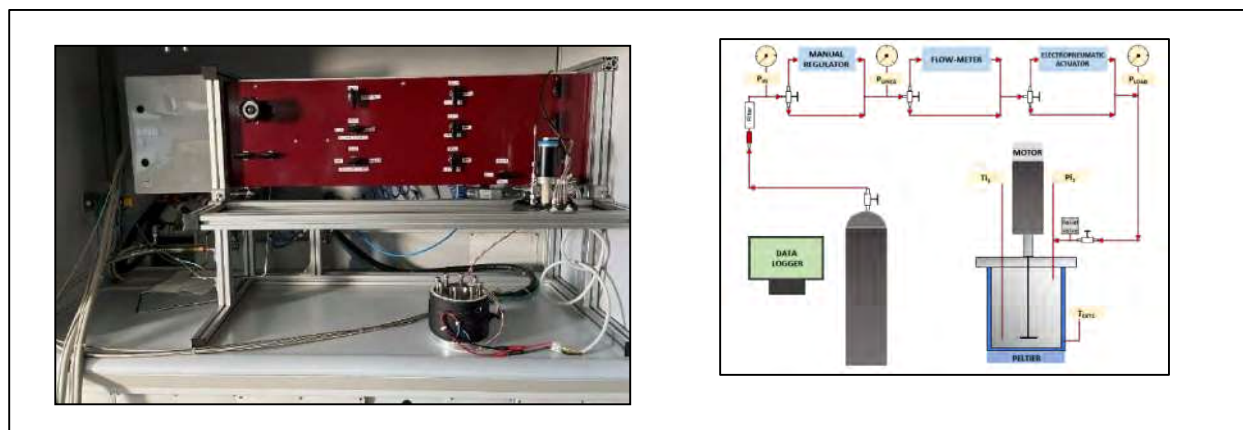
Figure 2. UniChieti lab-scale reactor.
