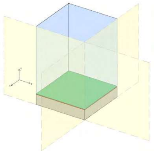
Figure 3. Model made in COMSOL Multiphysics.
