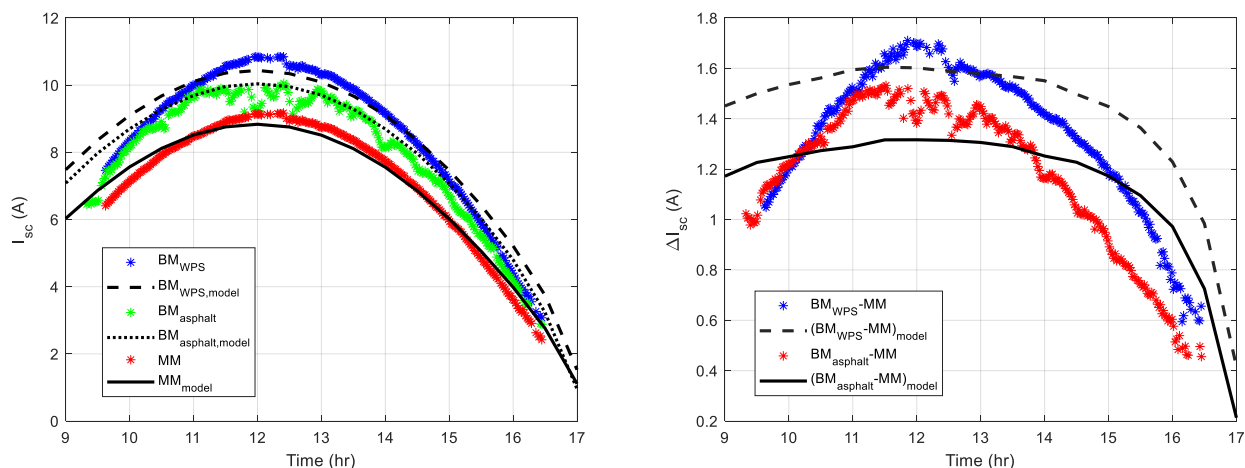
Figure 3. Comparison between the experimental and predicted values of short-circuit current of the monofacial mini-module and the bifacial-minimodules.
