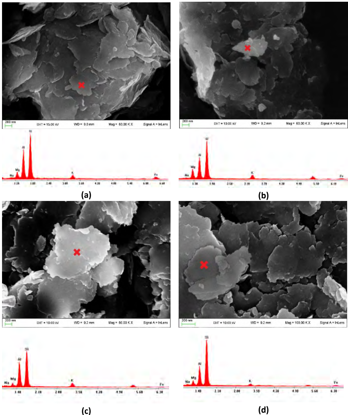
Figure 4. Fe-SEM photos of raw soils, PR/GRA (a), PR/OI (b), PR/PeA (c) and PR (d). For each photos the chemical analysis (EDS) was reported below, and the red cross indicates the point where analysis was carried out. The images show the typical lamellar structures of clay minerals.
