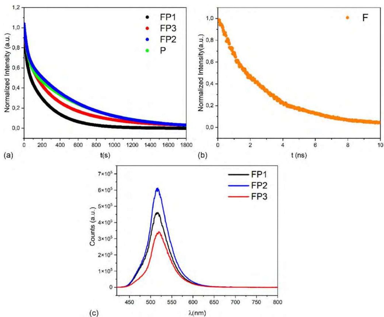
Figure 4. Luminescence decay profiles of (a) FP1, FP2, FP3, P and (b) F, monitored at \lambda_{\text{exc}} = 400 nm and \lambda_{\text{em}} = 510 nm. (c) Gated spectra of combined samples FP1, FP2 and FP3 samples ( \lambda_{\text{exc}} = 400 nm, delay time = 5 ms)
