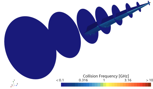
Fig. 4. Collision frequency at Mach 15 and 40 km altitude.
