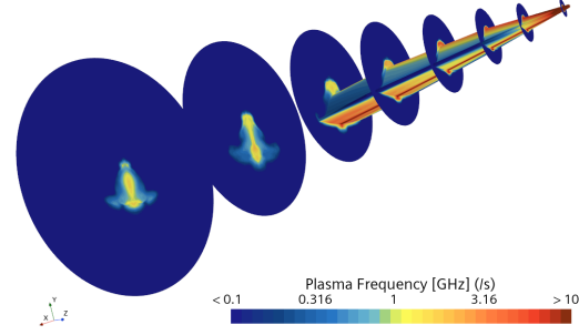
Fig. 3. Plasma frequency at Mach 15 and 40 km altitude.
