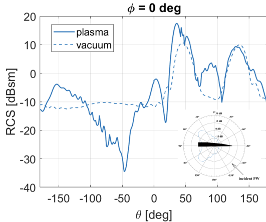
Fig. 7. Comparison of bistatic RCS with plasma and in vacuum.
