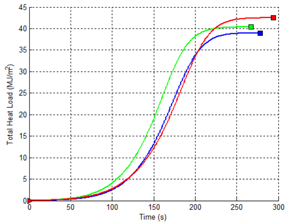
Fig. 9: IOD heat-load profile.
