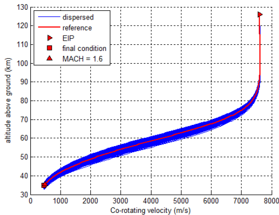
Fig. 11: IOD altitude vs velocity dispersion.
