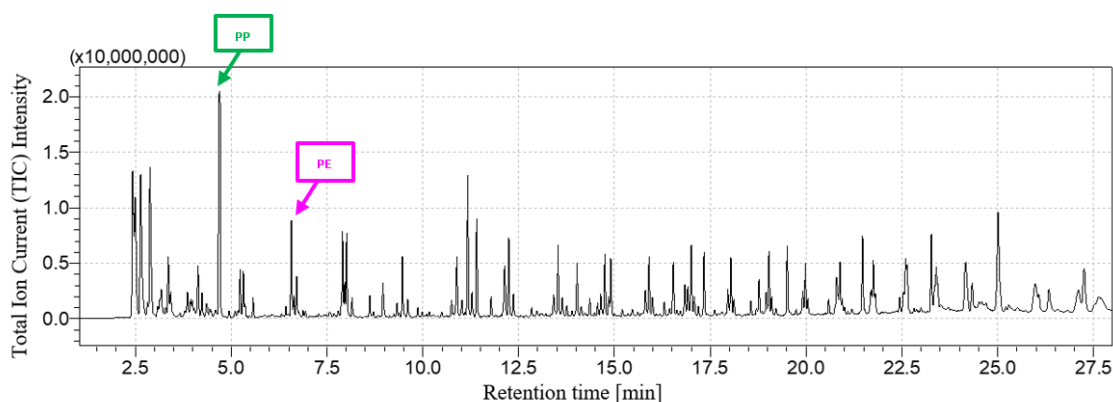
Figure 1. LDPE + PP chromatogram.
