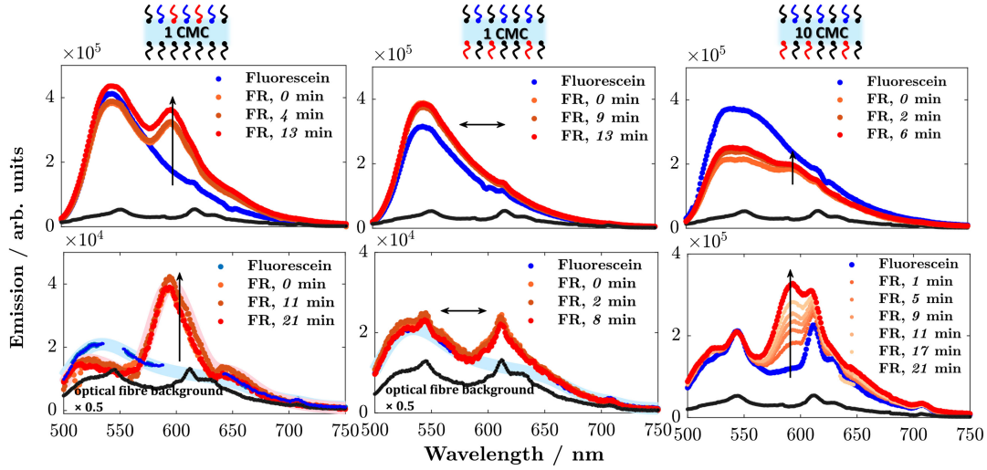
FIG. 2. Steady state luminescence data recorded for the amphiphilic dyes (10 \mu M solutions in the base surfactant) spray-doped on soap films of CTAC (top panel) and SDS (bottom panel) made from the same base surfactant. Excitation wavelength was 470 nm where the donor fluorescein was predominantly excited. Top left : Fluorescein and rhodamine sprayed on the same side of the soap film (base surfactant CTAC; concentration = 1.1 mM, 1 CMC). Immediate appearance of the rhodamine acceptor fluorescence peak at 590 nm clearly indicates the occurrence of FRET in the control, validating the method. Top middle : Fluorescein and rhodamine sprayed on different sides of the soap film (base surfactant CTAC, 1 CMC). Only fluorescein fluorescence ( \lambda_{\text{max}} \approx 535 nm) is observed; absence of any acceptor peak indicates persistent broken symmetry for at least 13 min, when the film broke. Top right : Fluorescein and rhodamine sprayed on different sides of the soap film (base surfactant CTAC; concentration = 11 mM, 10 CMC). Bottom panel : Same as the top panel, but with base surfactant SDS. Note : Signals in SDS are an order of magnitude lower than CTAC; the Fluorescein signal therefore nearly coincided with the background and has been plotted as a blue shaded line after correcting the data for background. SDS data at 10 CMC has been normalized to the fiber background at 540 nm for clearer depiction of the acceptor intensity increment.
