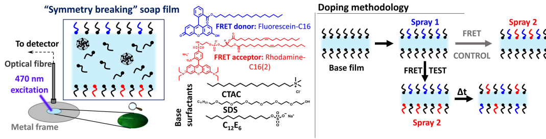
FIG. 1. Left : Molecular structures of amphiphilic fluorescein (blue), rhodamine (red), and different base surfactants (black) used in this study, together with a schematic depiction of the setup used for measurements and a cartoon depiction of the envisioned symmetry-breaking soap film. Right : Schematic depiction of the experiments used in this work to distinguish a symmetric and symmetry-breaking soap film.
