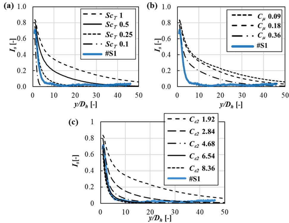
Fig. 6. Comparison between experimental, Case #S1 (solid blue line), and numerical segregation index profiles along the channel length evaluated for: (i) four different turbulent Schmidt numbers of: 1, 0.5, 0.25, 0.1 (Fig. 6.a); three C_\mu parameter values of: 0.09 (standard value), 0.18 and 0.36 (Fig. 6.b); and five C_{e2} values of: 1.92 (reference value), 2.84, 4.68, 6.54 and 8.36 (Fig. 6.c). In the latter case, the C_{e1} was always kept equal to 1.44 (default value).
