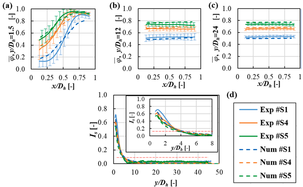
Fig. 7. (a)-(c): Experimental (solid lines) and numerical (dashed lines) time average mixture fraction profiles along the channel width at y/D_h equal to 1.5 (a), 12 (b) and 24 (c) for cases #S1 and the unbalanced operating conditions #S4 and #S5. (d) Experimental (solid lines) and numerical (dashed lines) segregation index profiles along the normalized channel locations. Vertical bars indicate the experimental time standard deviation of the mixture fraction values.
