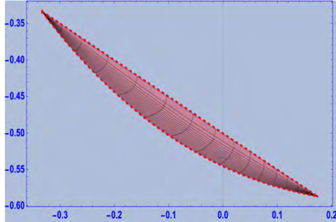
Figure 11. The plot of the map \Psi .
