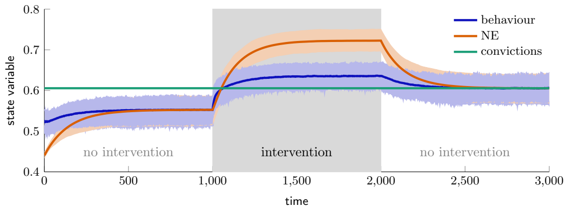
(b) \alpha = 0.58
