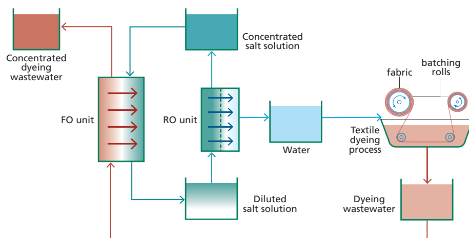
Figure 5 Implementing forward osmosis (FO) into the textile wastewater treatment process can provide high value to an industry segment which is a large consumer of fresh water and one of the biggest polluters. The scheme shows the FO process integrated in a textile wastewater treatment plant using inorganic salt as a draw solution. For using the salt solution as a draw solution there is an integrated reverse osmosis unit for the reuse of the diluted salt.
