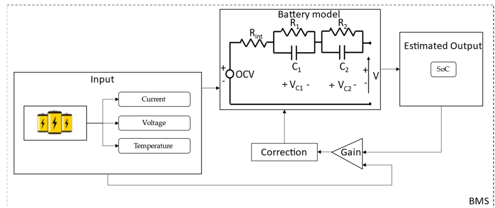
Figure 6. Kalman filter schematization for SoC estimation.
