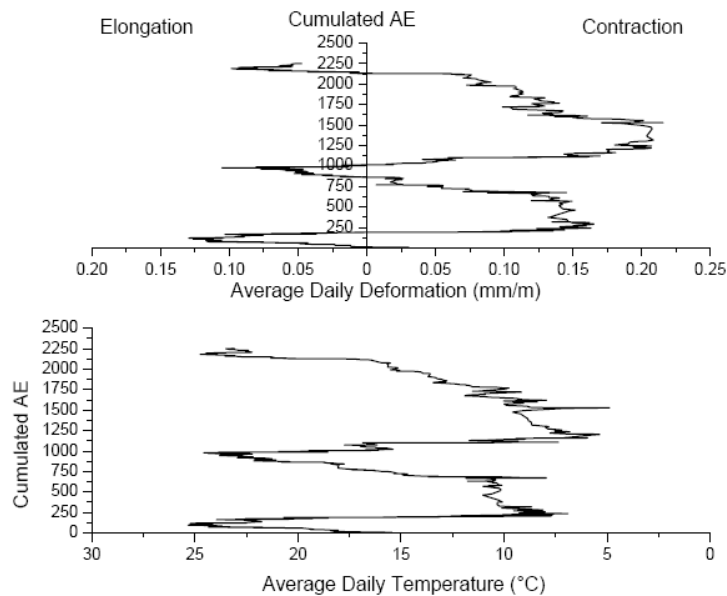
Figure 5: Correlation between cumulated AE activity vs FOS average daily deformations (up), and cumulated AE activity vs average daily temperature (down).
