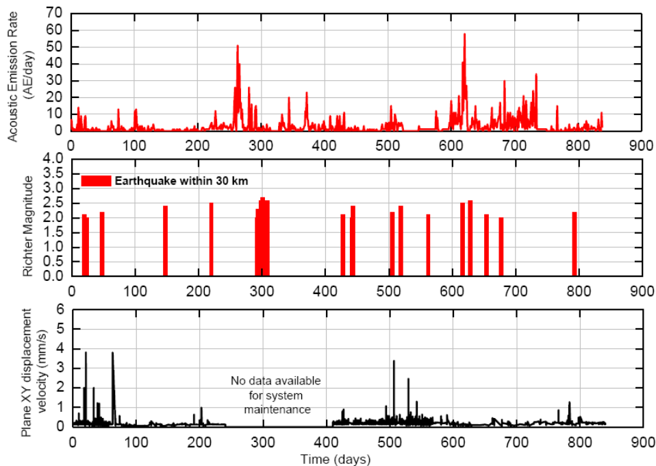
Figure 6: Rate trend of the AE signals during the entire monitoring period (up). Number of earthquakes, represented by their magnitude on the Richter scale, having their epicenters detected within a radius of 30 km from the city center of Bologna (middle). Speed of the transversal oscillations of the tower obtained by the seismometer (down).
