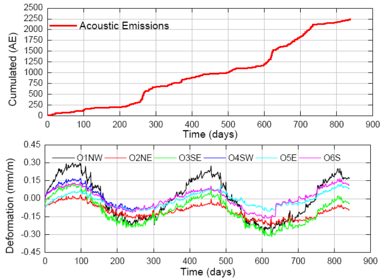
Figure 4: Trend of the cumulate function of the AE signals recorded by the 8 sensors (up), and daily deformations measured by means of the 6 optical strands (down).
