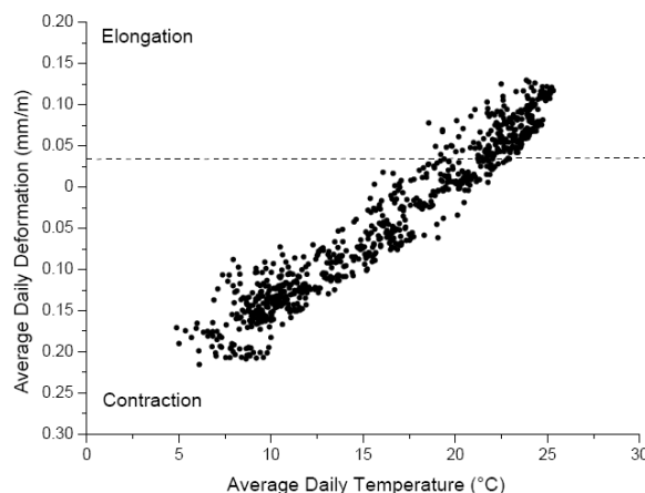
Figure 3: Correlation between walls average vertical deformations measured by FOS and tower internal temperature.
