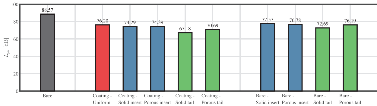
FIG. 9. Overall sound pressure level for the different cylinder configurations at Re_d = 4.1 \times 10^4 integrated between f = 131.25 and f = 20000 Hz. The L_{p0} values are indicated at the top of each bar. The notation for each cylinder configuration refers to Fig. 3(a).
