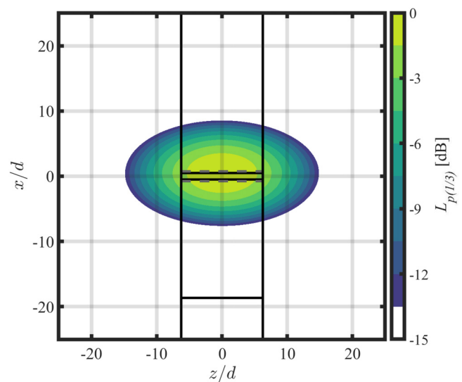
FIG. 5. Point-spread function at f_{1/3} = 1.6 kHz for a simulated source emitting white noise at the origin of the coordinate system. The flow goes from the bottom to the top of the map.
