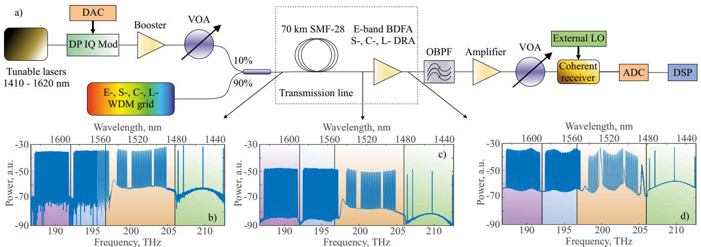
Fig. 3. a) Experimental setup of a B2B and transmission experiment; spectra of the WDM grid and E-band data carrier signal at 1457 nm at (b) input to the span, (c) end of the span, and (d) after the amplifier.
