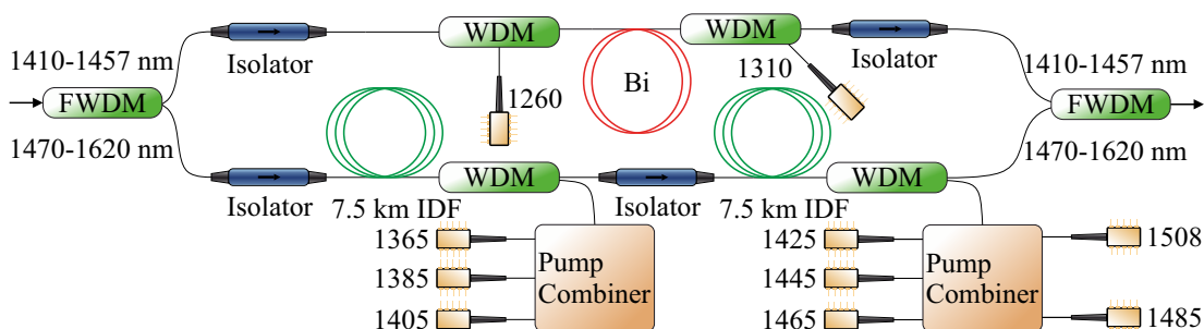
Fig. 1. Experimental setup of the ESCL-band amplifier used within this work, utilizing an active Bi-doped fiber and dual-stage discrete Raman amplification.
