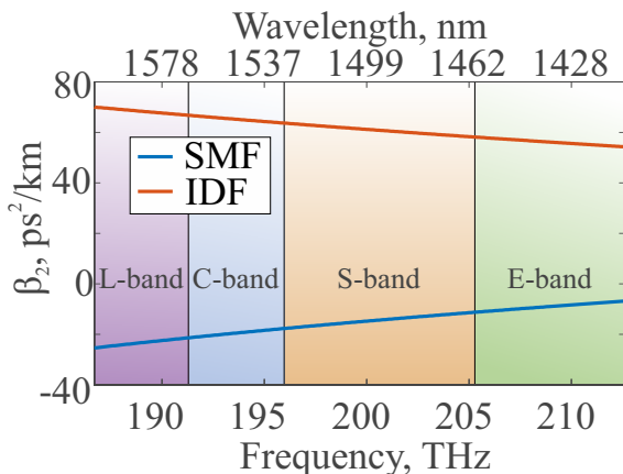
Fig. 6. The group velocity dispersion, \beta_2 , of SMF and IDF as a function of frequency in the ESCL-bands.
