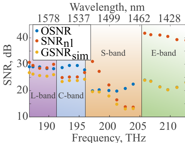
Fig. 11. The OSNR, SNR_{NL} , and GSNR_{SIM} values after propagation and amplification using the combined SCL-band Raman and the E-band BDFA.
