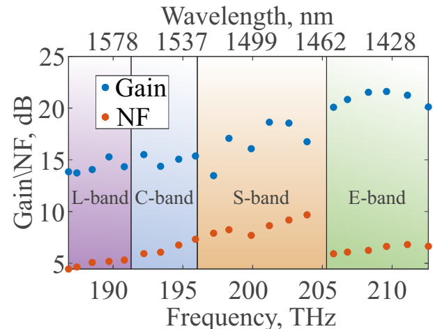
Fig. 9. The gain and NF profiles for the entire spectrum considered within the amplifier model.
