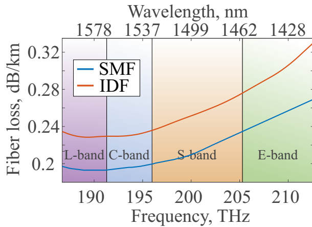
Fig. 5. The loss coefficients, \alpha , of the fibers used within this work as a function of frequency in the ESCL-bands.
