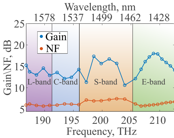
Fig. 2. Gain and NF of the developed ESCL-band amplifier
