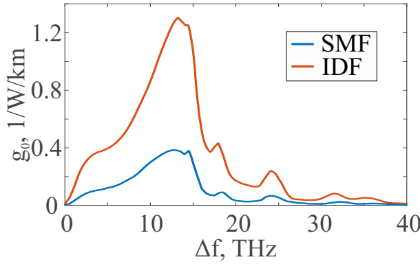
Fig. 8. The reference Raman gain coefficient, g_0 , corresponding to the Raman gain at a reference frequency, f_{\text{ref}} = 203.9 THz, for the two fibers used within this work, as a function of frequency.
