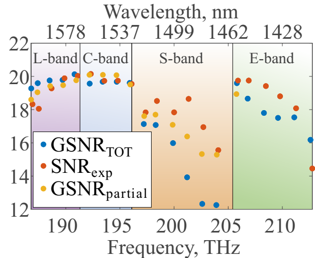
Fig. 12. The experimentally achieved SNR and numerically calculated GSNR values after propagation and amplification using the combined ESCL-band amplifier.
