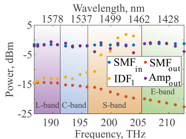
Fig. 10. The power profile of the signal at various points of transmission.
