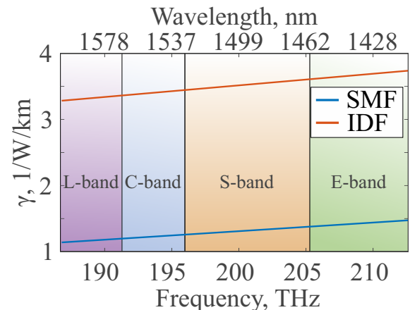
Fig. 7. The nonlinear coefficient, \gamma , of SMF and IDF as a function of frequency in the ESCL-bands.
