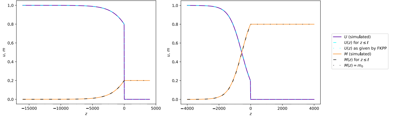
Figure 5: Numerical solutions of Equations (12)-(13) subject to the initial conditions (16)-(17), for m_0 = 0.2 on the left and m_0 = 0.8 on the right with rescaled ECM degradation rate \lambda = 10^{-3} translated into the travelling wave co-ordinate, z . Solid lines represent the cell and ECM densities from numerical simulations in purple and orange respectively. The FKPP solution (42) in travelling wave co-ordinates is plotted as a dotted blue line. The solution M(z) = m_0 is plotted in dotted black, and the analytical solutions given by Equations (48) and (49) are plotted in dashed blue and black lines, respectively. Further specifics of the parameter values and the numerical methods used can be found in Appendix B.
