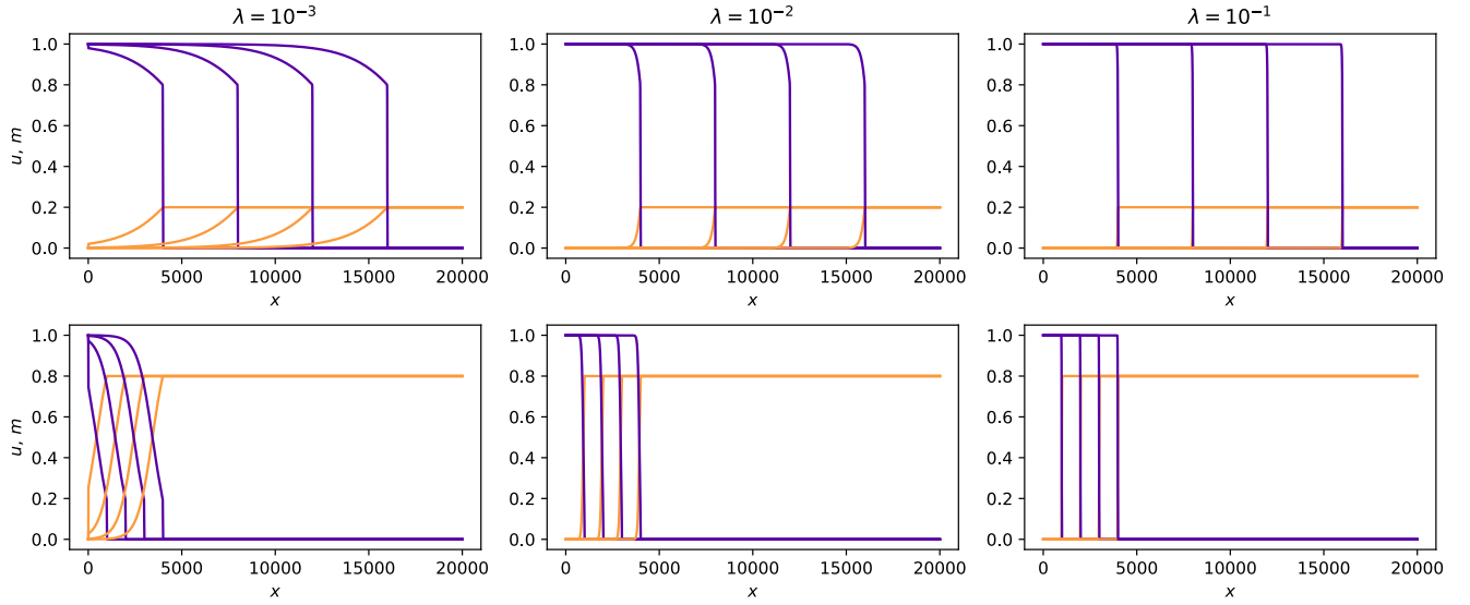
Figure 4: Numerical solutions of Equations (12)-(13) subject to the initial conditions (16)-(17), for m_0 = 0.2 in the top row and m_0 = 0.8 in the bottom row, and for rescaled ECM degradation rates \lambda = 10^{-3}, 10^{-2}, 10^{-1} . Cell densities are shown in purple and ECM densities in orange at times t = 2500, 5000, 7500, 10000 from left to right. Further specifics of the parameter values and the numerical methods used can be found in Appendix B.
