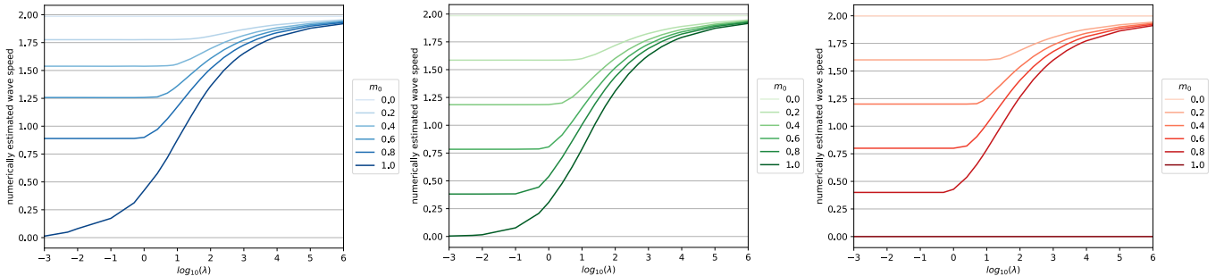
Figure 9: The relationship between the numerically estimated speed of travelling wave solutions to the system (62)-(63) on the left (blue), (64)-(65) in the middle (green) and (12)-(13) on the right (red), subject to the initial conditions (16)-(17). The numerically estimated travelling wave speed is obtained by tracing the point X(t) such that u(X(t), t) = 0.1 . Further specifics of the parameter values and the numerical methods used can be found in Appendix B.
