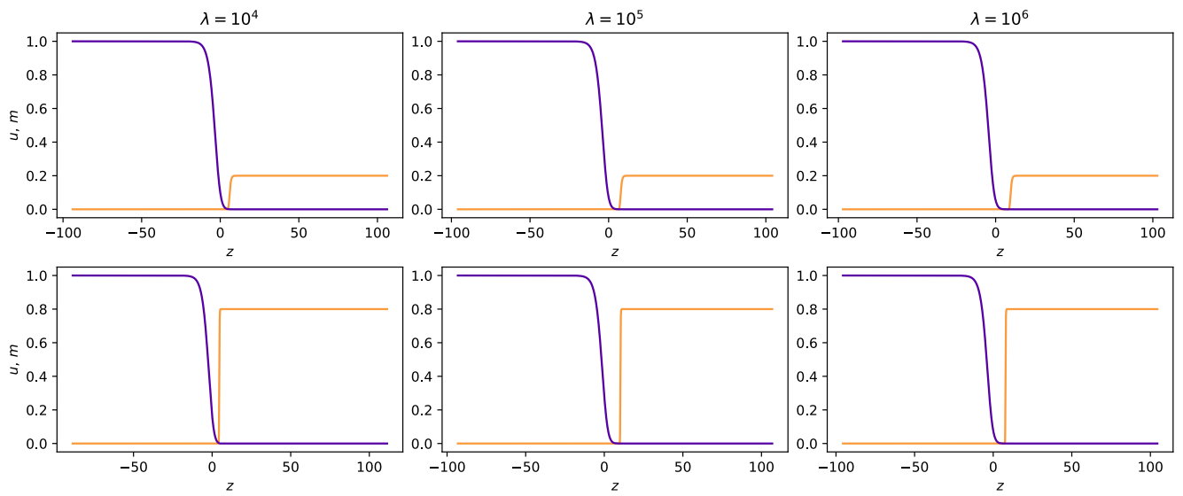
Figure 12: Travelling wave solutions of Equations (12)-(13) subject to the initial conditions (16)-(17), for m_0 = 0.2 in the top row and m_0 = 0.8 in the bottom row, and for rescaled ECM degradation rates \lambda = 10^4, 10^5, 10^6 . Cell densities are shown in purple and ECM densities in orange. Further specifics of the parameter values and the numerical methods used can be found in Appendix B.
