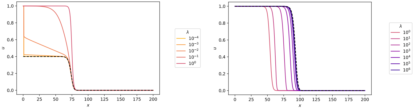
Figure 6: Left: plot of the cell density, u , obtained through numerical simulations of Equations (12)-(13) subject to the initial conditions (16)-(17) (solid lines) for small values of \lambda , and numerical simulations of the FKPP model (11) with rescaled coefficients \hat{D} = \hat{r} = \hat{K} = 1 - m_0 (dashed black line) with t = 100 and m_0 = 0.6 . Right: plot of the cell density, u , obtained through numerical simulations of Equations (12)-(13) subject to the initial conditions (16)-(17) (solid lines) for large values of \lambda , and numerical simulations of the FKPP model (18) (dashed black line) in the plot on the right for t = 50 and m_0 = 0.4 . Qualitatively, the same behaviour is observed for all m_0 \in [0, 1) . Further specifics of the parameter values and the numerical methods used for the simulations can be found in Appendix B.
