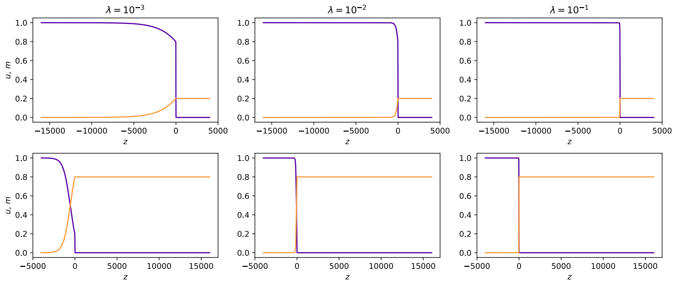
Figure 10: Travelling wave solutions of Equations (12)-(13) subject to the initial conditions (16)-(17), for m_0 = 0.2 in the top row and m_0 = 0.8 in the bottom row, and for rescaled ECM degradation rates \lambda = 10^{-3}, 10^{-2}, 10^{-1} . Cell densities are shown in purple and ECM densities in orange. Further specifics of the parameter values and the numerical methods used can be found in Appendix B.
