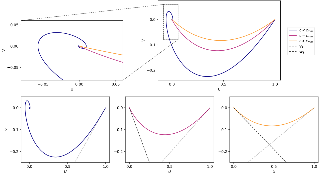
Figure 3: Phase plane plot of the ODE system (29)-(30), for different travelling wave speeds, c , demonstrating the change from a stable spiral to a stable node as the travelling wave speed exceeds c_{min} . The corresponding unstable eigenvector given by Equation (36) and stable eigenvector given by Equation (39) are overlaid in the lower plots [30]. Further specifics of the parameter values and the numerical methods used can be found in Appendix B.
