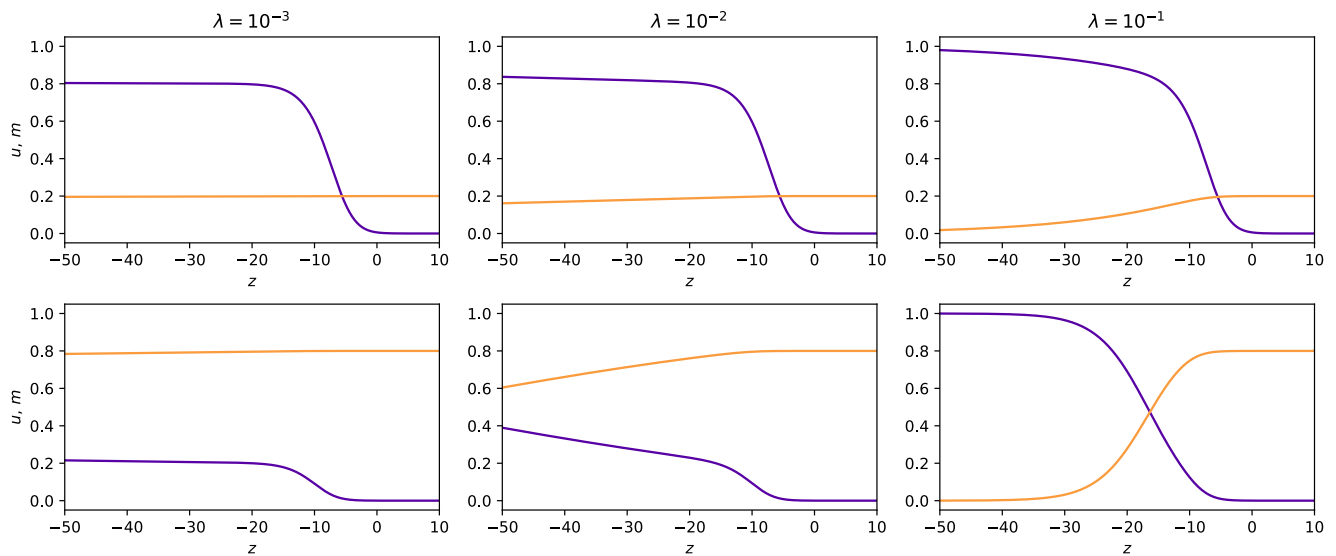
Figure 11: Travelling wave solutions of Equations (12)-(13) subject to the initial conditions (16)-(17), for m_0 = 0.2 in the top row and m_0 = 0.8 in the bottom row, and for rescaled ECM degradation rates \lambda = 10^{-3}, 10^{-2}, 10^{-1} . Cell densities are shown in purple and ECM densities in orange, zoomed in on the evolved travelling wave front, as shown in Figure 10. Further specifics of the parameter values and the numerical methods used can be found in Appendix B.
