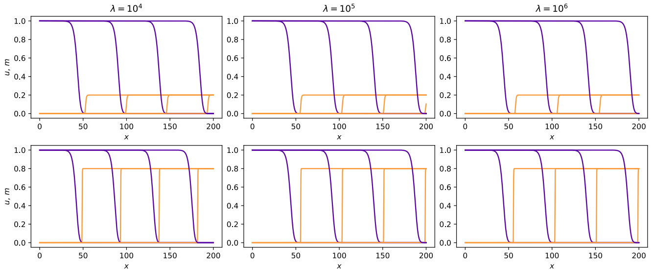
Figure 7: Numerical solutions of Equations (12)-(13) subject to the initial conditions (16)-(17), for m_0 = 0.2 in the top row and m_0 = 0.8 in the bottom row, and for rescaled ECM degradation rates \lambda = 10^4, 10^5, 10^6 . Cell densities are shown in purple and ECM densities in orange at times t = 25, 50, 75, 100 from left to right. Further specifics of the parameter values and the numerical methods used can be found in Appendix B.
