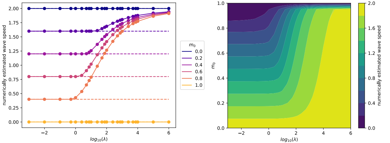
Figure 2: The relationship between the numerically estimated speed (solid lines) of travelling wave solutions of Equations (12)-(13) subject to the initial conditions (16)-(17). The dashed lines in the plot on the left highlight the value of 2(1 - m_0) . The numerically estimated travelling wave speed is obtained by tracing the point X(t) such that u(X(t), t) = 0.1 . Further specifics of the parameter values and the numerical methods used can be found in Appendix B.
