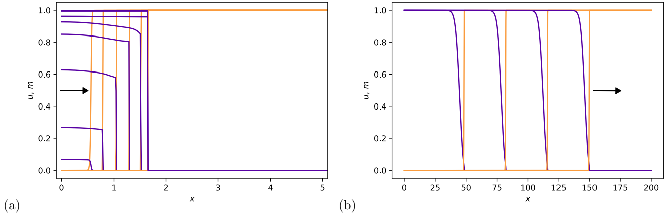
Figure 8: Numerical solutions to the system (12)-(13) subject to the initial conditions (53) and (54) (panel (a)) or (53) and (55) (panel (b)), for m_0 = 1 and \lambda = 250 . Cell densities are shown in purple and ECM densities in orange at times t = 2, 4, 6, 8, 10, 12, 14, 16 (from left to right) in panel (a) and times t = 25, 50, 75, 100 (from left to right) in panel (b). Note that the axis in the plot in panel (a) are zoomed in on x \in [0, 5] to display the initial behaviour in the transient region before invasion stops. Further specifics of the parameter values and the numerical methods used for simulation can be found in Appendix B.
