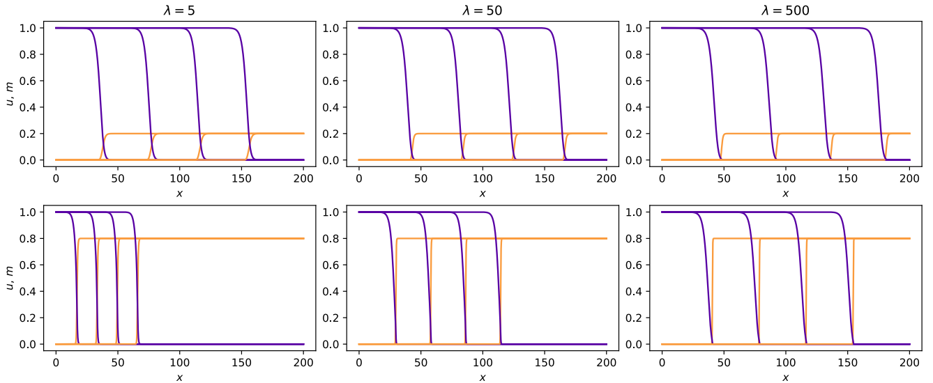
Figure 1: Numerical solutions of Equations (12)-(13) subject to the initial conditions (16)-(17), for m_0 = 0.2 in the top row and m_0 = 0.8 in the bottom row, and for rescaled ECM degradation rates \lambda = 5, 50, 500 . Cell densities are shown in purple and ECM densities in orange at times t = 25, 50, 75, 100 from left to right. Further specifics of the parameter values and the numerical methods used can be found in Appendix B.
