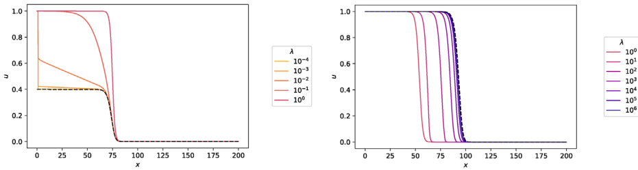
FIGURE 6 Left: plot of the cell density, u , obtained through numerical simulations of Equations (12) and (13) subject to the initial conditions (16) and (17) (solid lines) for small values of \lambda , and numerical simulations of the FKPP model (11) with rescaled coefficients \hat{D} = \hat{f} = \hat{K} = 1 - m_0 (dashed black line) with t = 100 and m_0 = 0.6 . Right: plot of the cell density, u , obtained through numerical simulations of Equations (12) and (13) subject to the initial conditions (16) and (17) (solid lines) for large values of \lambda , and numerical simulations of the FKPP model (18) (dashed black line) in the plot on the right for t = 50 and m_0 = 0.4 . Qualitatively, the same behavior is observed for all m_0 \in [0, 1) . Further specifics of the parameter values and the numerical methods used for the simulations can be found in Appendix B.
