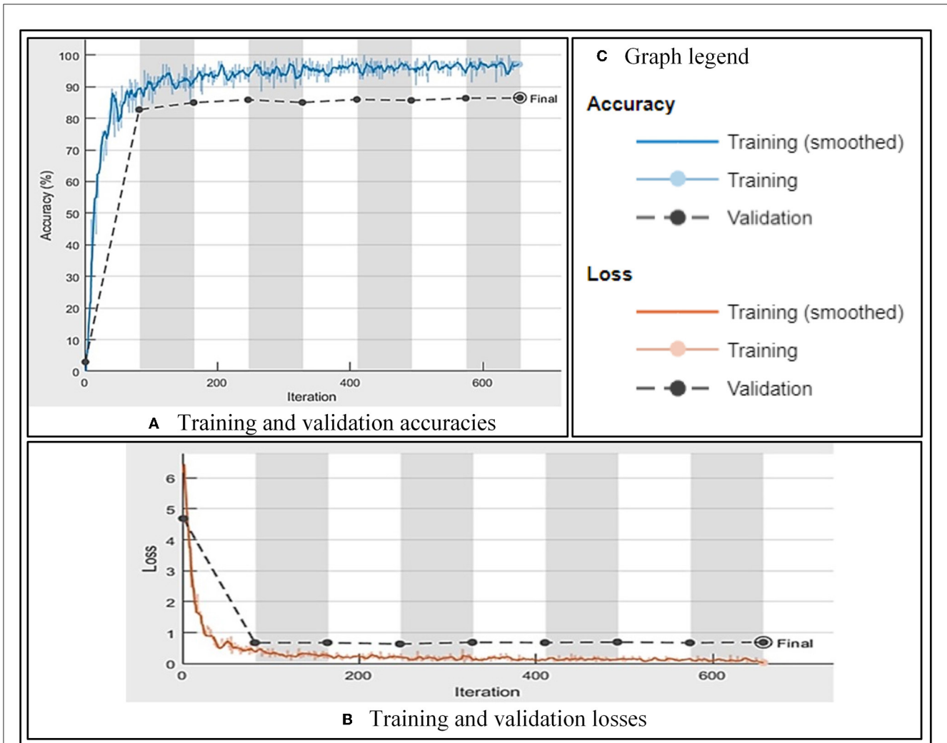
FIGURE 4 FRAI training and validation performance. (A) Training and validation accuracies. (B) Training and validation losses. (C) Graph legend.
