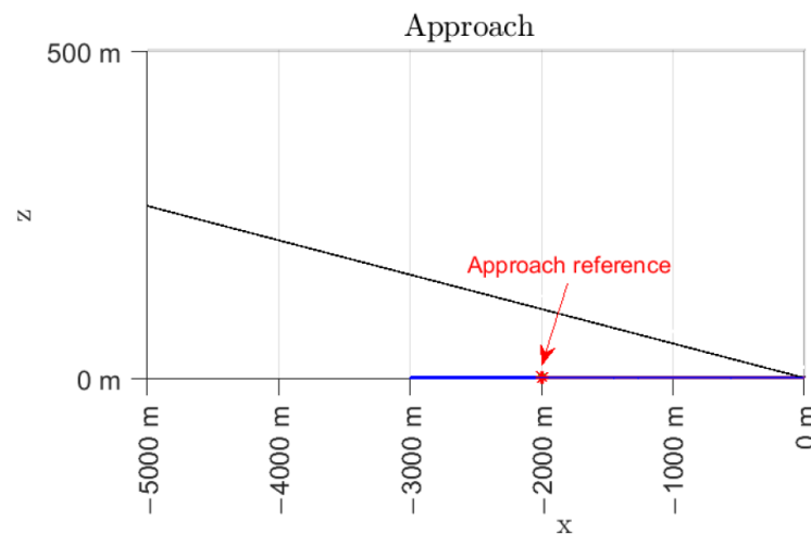
Figure 9. Simulated approach flight path.
