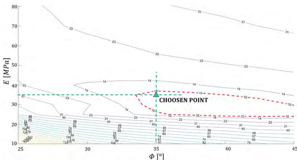
Figure 9. Mean absolute percentage error (MAPE) in the calibration of the soil mechanical parameters by PLT data.
