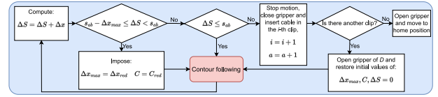
Fig. 9: Flowchart of the cable routing skill.
