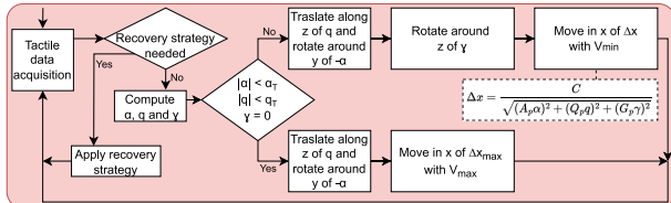
Fig. 8: Flowchart of the contour following skill.
