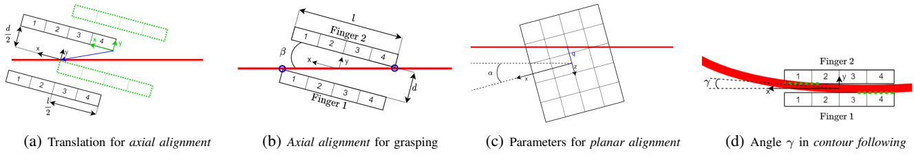
Fig. 4: Schematic representations of several configurations of the DLO (in red) and the fingertips equipped with tactile sensors. The x , y and z axes reported belong to the tool reference frame.
