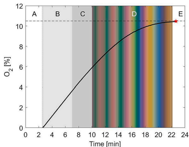
Fig. 7. Experimental dioxygen diffusion and related color patterns for the C_{12}E_6 surfactant at 10 CMC concentration. The reported time spans correspond to: dioxygen purging (A); transparent soap film (B); rapidly-changing colors (C); smooth color changing (D) and bursting of the soap film (E). The dioxygen data acquisition starts at 2 min 34 s. The horizontal dashed line indicates the final dioxygen concentration, expected at 10.5%. The red pentagram pinpoints the observed bursting condition of the soap film. (For interpretation of the references to color in this figure legend, the reader is referred to the web version of this article.)
