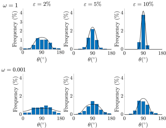
Fig. 6 Equilibrium distributions (16) changing \bar{\sigma} , \omega and \varepsilon , while \sigma = 0.2 everywhere. The parameter \varepsilon = 2\% , 5\% , 10\% (first, second and third columns, respectively) is changed according to the experimental setup giving rise to decreasing values of \bar{\sigma}^2 = \frac{\sigma^2}{2\varepsilon^2} in the first row and \bar{\sigma}^2 = \frac{\sigma^2}{2\varepsilon^2\lambda\omega} with \lambda = 100 s in the second row. The value of \bar{K}_s = 0.7 is used.
