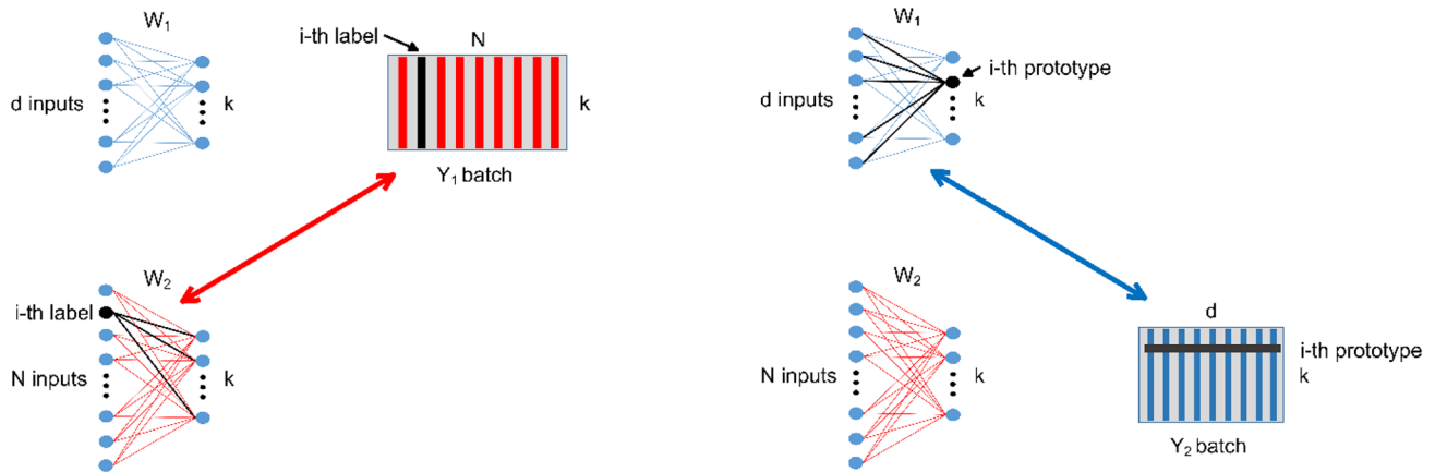
Fig. 3 Half dualities
