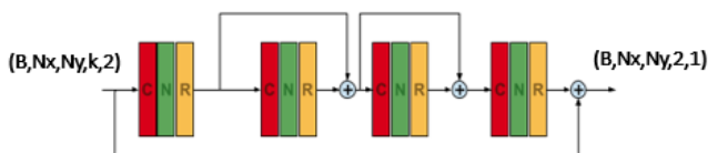
Fig. 2. Neural network architecture, channel last convention.
