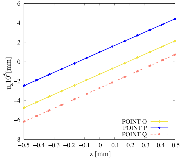
(a) u_z along the thickness.
