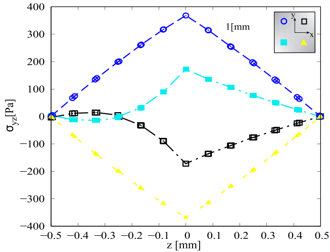
Fig. 15. \sigma_{yz} calculated in four points in the quarters of the plate. 22 \times 22 Q9, 4LE3. \theta = 1^\circ , simply supported GFRP VAT plate [2(0 < 90, 60 >), 2(0 < 45, 0 >)] .
