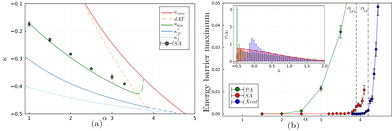
FIG. 3. (a) Coalescence threshold lines at \kappa_E = -0.5 (blue and cyan), and the \kappa_{kern} threshold (green line) as a function of \alpha . In orange the dAT transition line, delimiting the RS-stable region; in red the RS estimate of the \kappa_{max} . Above the dAT line, dashed lines indicate the continuation of the (unstable) RS predictions. Points are numerical extrapolations from SA samples (see SM for details). (b) Maximum error along the geodesic path ( y = 2 ) connecting numerical solutions found with different algorithms (PA, SA, and Xent) with the fBP max-margin solutions. Nonzero energies along the path indicate disconnection in the solution space. The vertical dashed lines denote the values of \alpha_{dAT} and \alpha_{LE} at \kappa_E = -0.5 . The inset shows stability distributions for PA, SA, and Xent at \alpha = 2 compared with the theoretical stability distribution of typical solutions (red dashed line).
