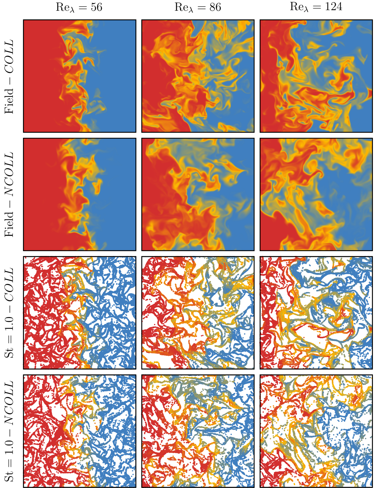
Figure 1: Visualization of fluid fields and suspended particles at \text{St} = 1 in a small slab around a (x_1, x_3) plane after three eddy turnover times \ell/u' in collisional and collisionless regimes at different \text{Re}_\lambda . Particles, out of scale, are coloured according to their temperature, the red colour denotes the highest temperature in the domain, and the blue colour the lowest temperature.
