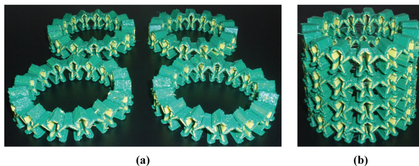
Figure 12 3D printed replicas of the single-module NPR jounce bumper (a); four stacked modules of the NPR ring (b)
