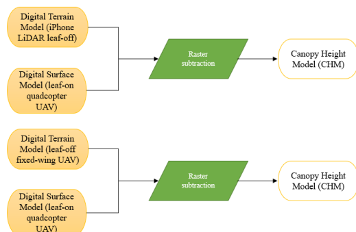
Figure 7: CHMs from the integration of iPhone LiDAR and UAV photogrammetry
