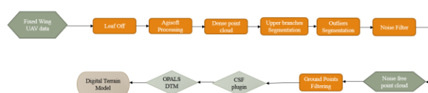
Figure 5: Methodology for generation of DTM from Leaf-off datasets
