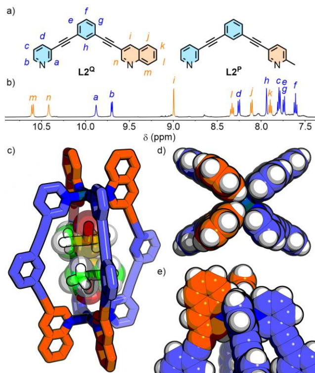
Fig. 4 a) Ligands L2^Q and L2^P ; b) Partial ^1H NMR (500 MHz, d_6 -DMSO, 298 K) of C2^Q ; SCXR structure of cis - C2^Q showing c) cis - C2^Q →DMSO 2 , d) view down Pd...Pd axis, and e) cis coordination environment around a Pd(II) ion.
