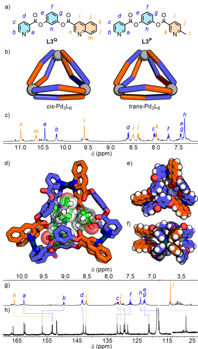
Fig. 5 a) Ligands L3^Q and L3^P ; b) cartoons of Pd_3L_6 'double-walled' triangle isomers with all- cis and all- trans donor arrangements; c) ^1H NMR (500 MHz, d_6 -DMSO) of C3^Q ; SCXR structure of cis - C3^Q showing d) cis - C3^Q →DMF 2 DMSO, and space filling representation e) from the top, and f) from the side; g) ^1H NMR (500 MHz, CD_3CN ) and h) ^{13}C NMR (126 MHz, CD_3CN ) of C3^P .
