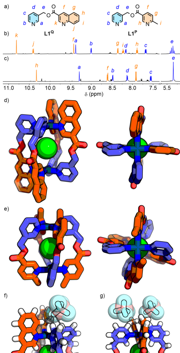
Fig. 2 a) Ligands L1^Q and L1^P . Partial 1 H NMR (500 MHz, d 6 -DMSO, 298 K) of b) C1 Q , and c) C1 P . SCXRD structures of d) cis - C1 Q ·Cl (only one crystallographically independent conformer shown), and e) trans - C1 P ·Cl. Exohedral interactions of BF 4 - counteranions with the Pd(II) coordination sphere in f) C1 Q (F...H 2.31-2.45 Å, C-H...F 139-156°), and g) C1 P .
