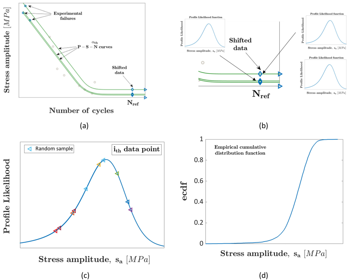
Figure 1. Proposed statistical method accounting for the uncertainty associated with the fatigue response of AM specimens: (a) procedure for shifting the experimental failures to the N_{ref} ; (b) Profile Likelihood functions for the fatigue strengths shifted at N_{ref} ; (c) random fatigue strength extraction by considering the estimated Profile Likelihood functions; (d) example of the empirical cumulative distribution function (ecdf) describing the fatigue strength distribution at N_{ref} .
