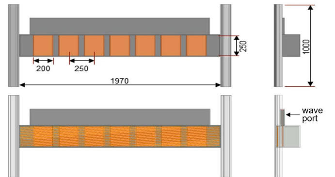
Figure 2. TWA model used in the simulation with main dimensions expressed in mm. The two models, respectively with and without a Faraday screen, are presented. The wave port used in the HFSS model is also illustrated.
