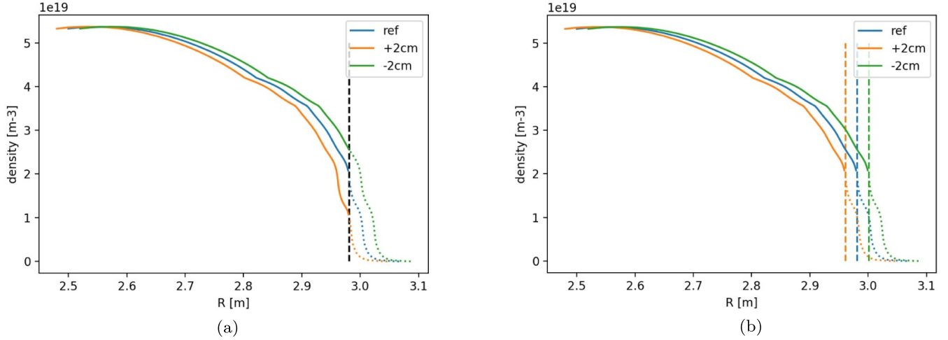
Figure 8. (a) Shifting the density profile and keeping the LCFS distance cut to the antenna. The LCFS cut is presented in black on the figure. (b) Shifting the entire profile from the antenna. The second option was used to test the TWA sensitivity to load variations.
