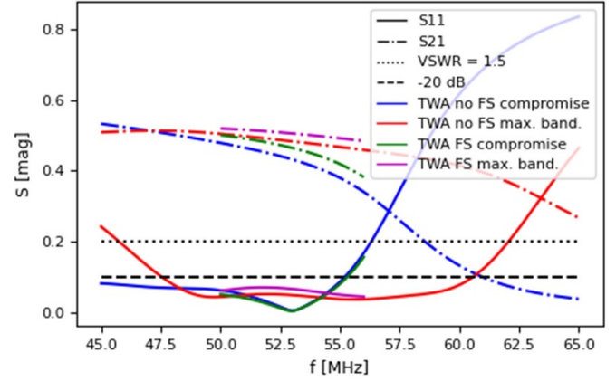
Figure 11. TWA frequency responses for the two capacitor layouts: a TWA tuned to have the maximum frequency bandwidth around 53 MHz or the engineering compromise reducing the antenna fields and power spectrum.
