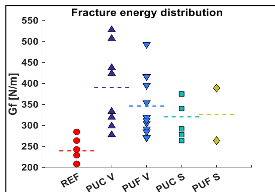
Fig. 10. Fracture energy distribution of all the specimens
