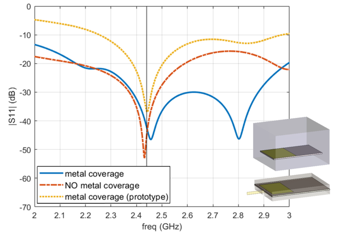
Fig. 4. Modulus of the S11 parameter as a function of frequency for different optimized configurations. The inset shows the optimized initial ( top ) and realizable ( bottom ) layouts.
