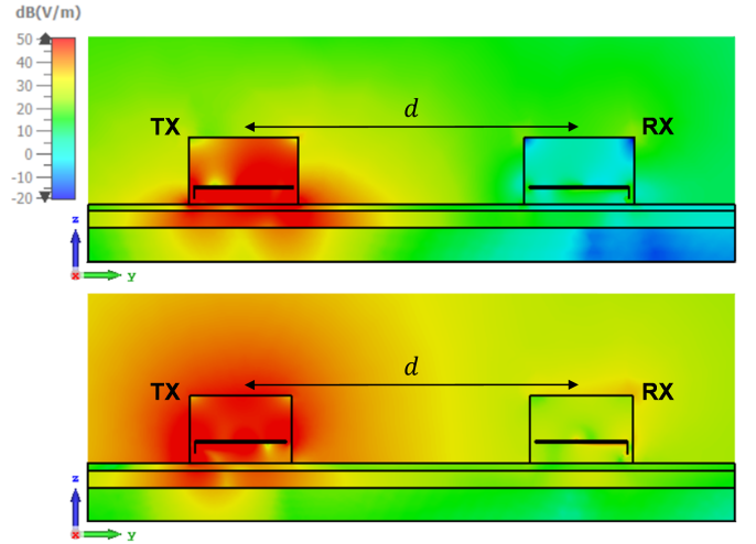
Fig. 3. Electric field magnitude for the optimized printed monopole antenna embedded into the coupling brick in the presence ( upper row ) and in the absence ( lower row ) of the metal coverage.
